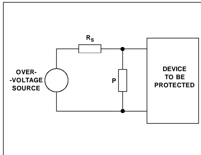
Figure1 : Classical schematic of parallel protection
