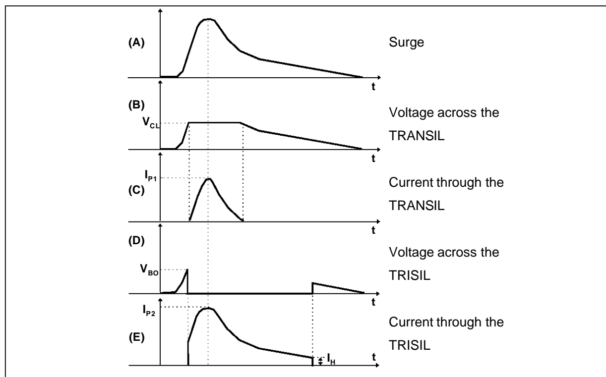
Figure 3 : Electrical behaviour in a Transil and a Trisil
