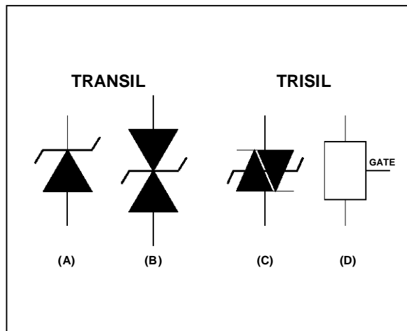
Figure 2 : Electrical Schematics
