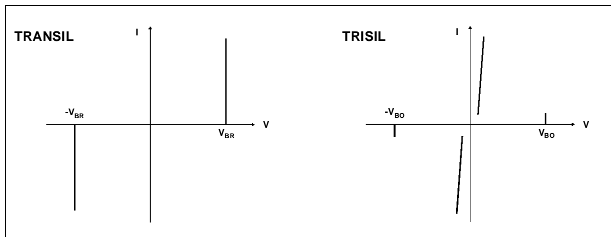
Figure 1 : Electrical characteristics
